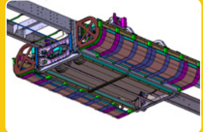
Four CNG tanks (60 diesel gallon equivalent).
